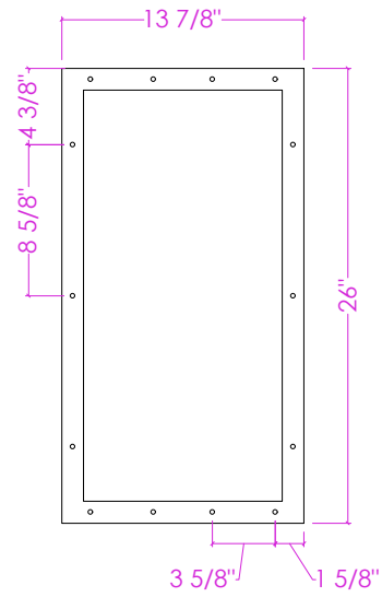
Back bracket
