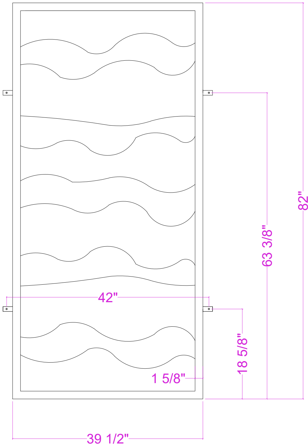
Blue Wave Ladder Gym-Style Climbing Wall Panel System
