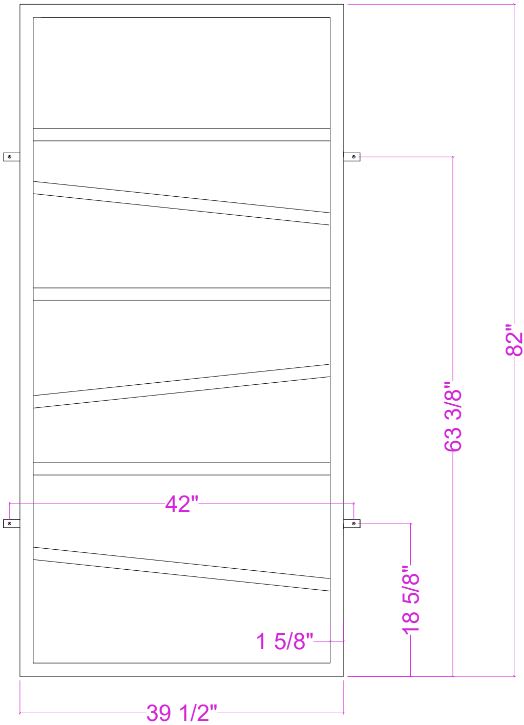
Slanted Bars Ladder Climbing Wall Panel - Wood Frame
